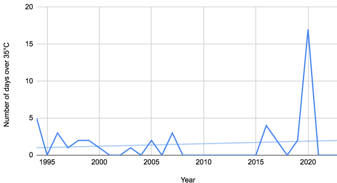
Luanda: Number of days over 35°C/year
